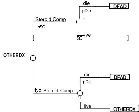
FIGURE 4. OTHERDX cycle tree. The possible transitions between OTHERDX and other states are shown. The probability of death is modified in the upper branch with a regular binding expression (not shown). Other abbreviations as in previous figures.
