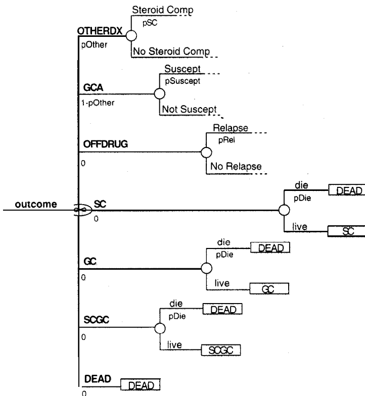
FIGURE 3. Markov subtree "outcome." A Markov subtree consists of a Markov node (indicated by the oval with the infinity symbol) and its branches, which represent the states of the Markov process. In the process represented by the "outcome" subtree, there are seven states: OTHERDX, GCA, OFFDRUG, SC, GC, SCGC, and DEAD (see text for descriptions of these states). The probability value beneath each branch indicates the fraction of the cohort initially in that state. Special binding expressions for the variables m.UINIT, m.UINCR, and m.UTAIL, are located on each branch but are not illustrated. Each branch is connected to a cycle tree that indicates the transitions between states during a given cycle (see figs. 4,5, and 6). OTHERDX, GCA, OFFDRUG, SC, GC, SCGC, and DEAD = states of the Markov process; Steroid Comp = steroid complication; pSC = probability of a steroid complication per cycle; Suscept = susceptibility to a GCA complication; pSuscept = probability of being susceptible to a GCA complication; Relapse = relapse of acute GCA; pRel = probability of acute GCA relapse per cycle; pDie = probability of death. Other abbreviations as in figure 2.
